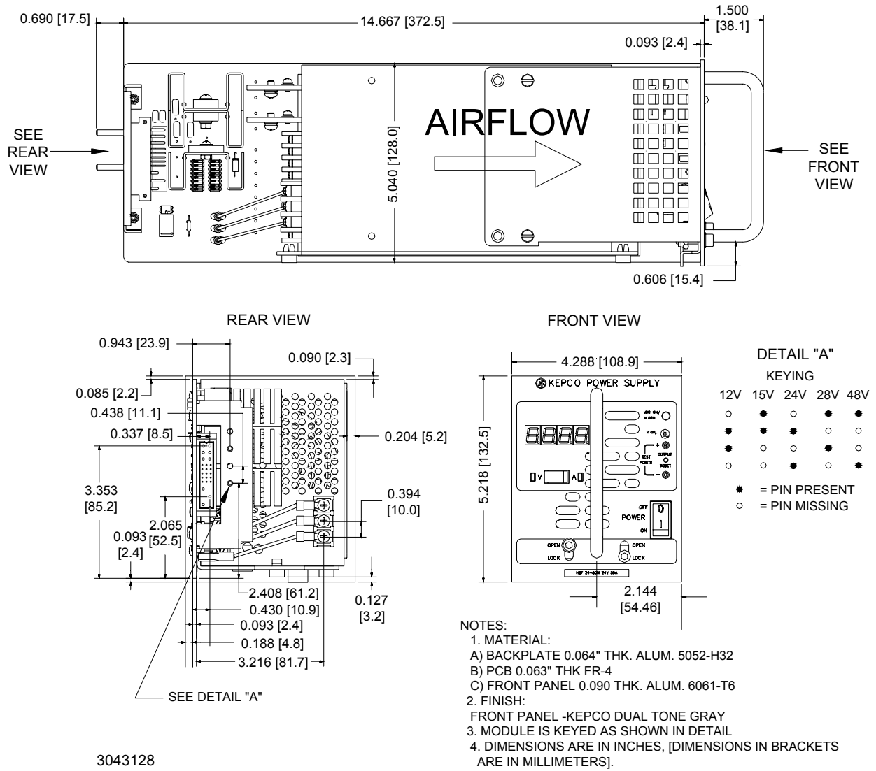
FIGURE 3. MECHANICAL OUTLINE DRAWING OF THE HSF (M) 600W POWER SUPPLY
