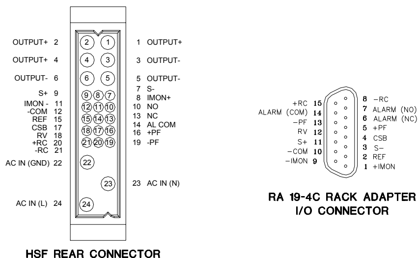
FIGURE 1. HSF (M) REAR PANEL CONNECTOR AND RA 19-4C RACK ADAPTER I/O CONNECTOR
